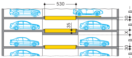
Intermediate slab
