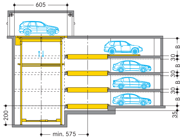
Intermediate slab
